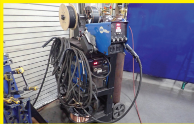
MILLER XMT-350
