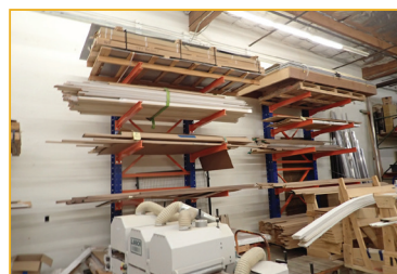
DOUBLE SIDED CANTILEVER RACKS
