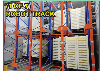
155'X20'H DOUBLE ROW 3-TIER HIGH DENSITY PALLET RACKING
